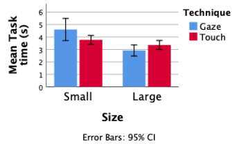
Figure 6: Mean task completion times
